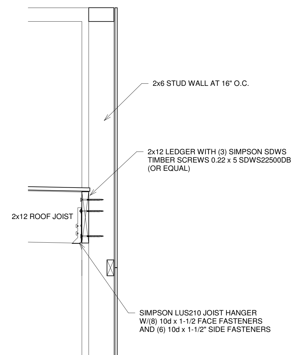
5 BALCONY FLOOR JOISTS SCALE: 1" = 1'-0"
