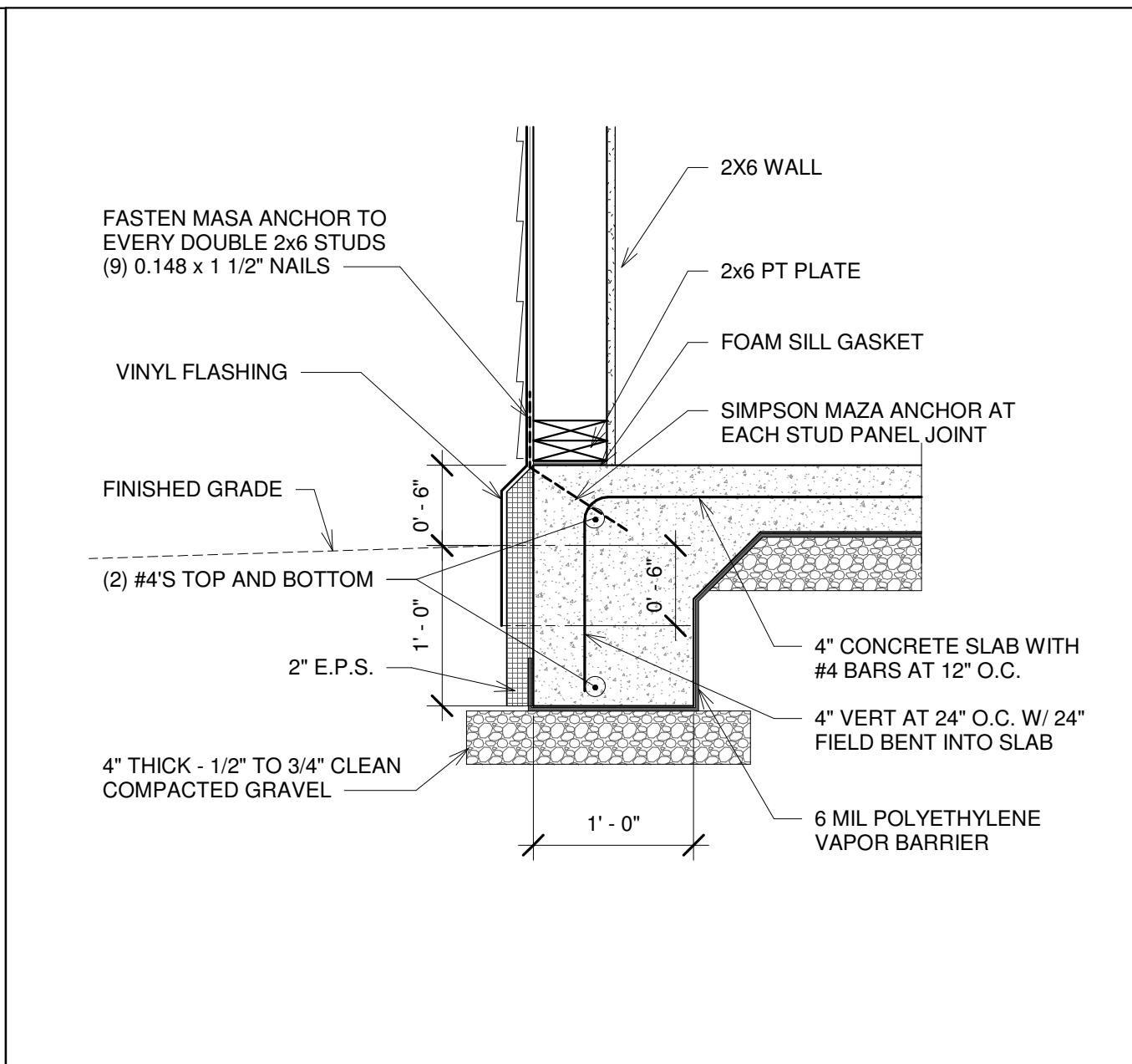
4 TYPICAL EXTERIOR FOOTING SCALE: 1" = 1'-0"
