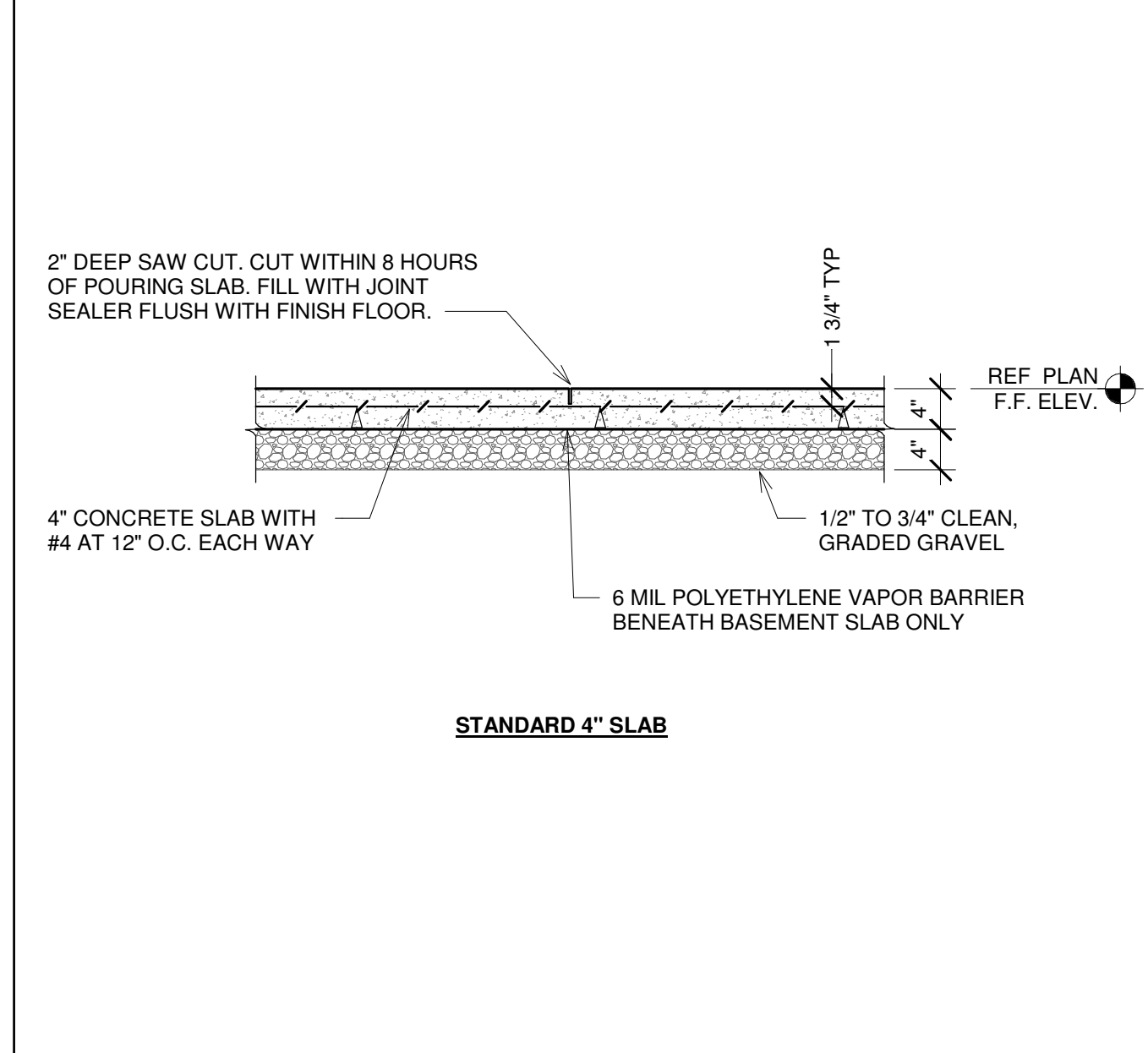
2 STANDARD SLAB DETAILS SCALE: 3/4" = 1'-0"
