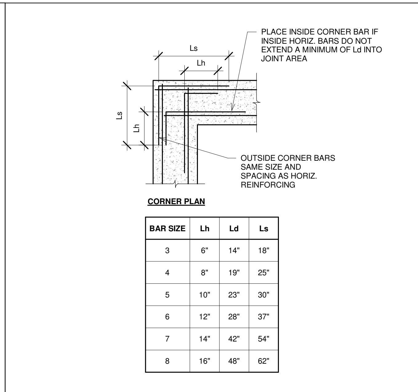
3 TYP WALL AND GRADE BEAM DETAILS SCALE: 3/4" = 1'-0"
