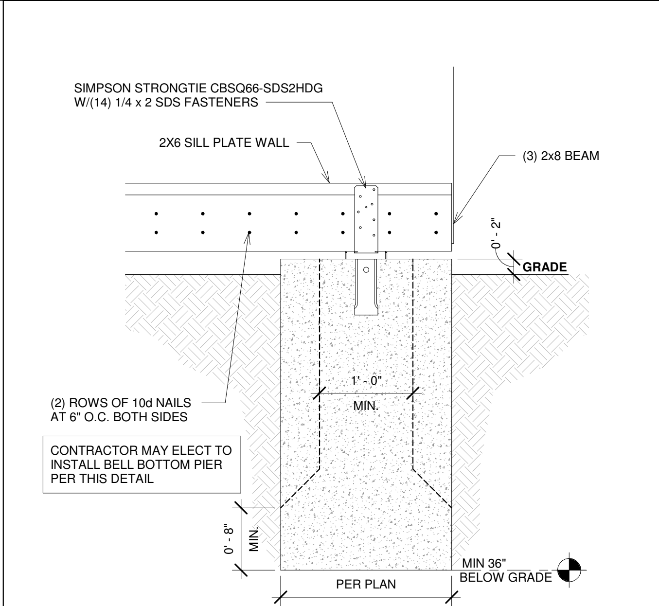
6 ENTRY CARPORT PIER SCALE: 1" = 1'-0"
