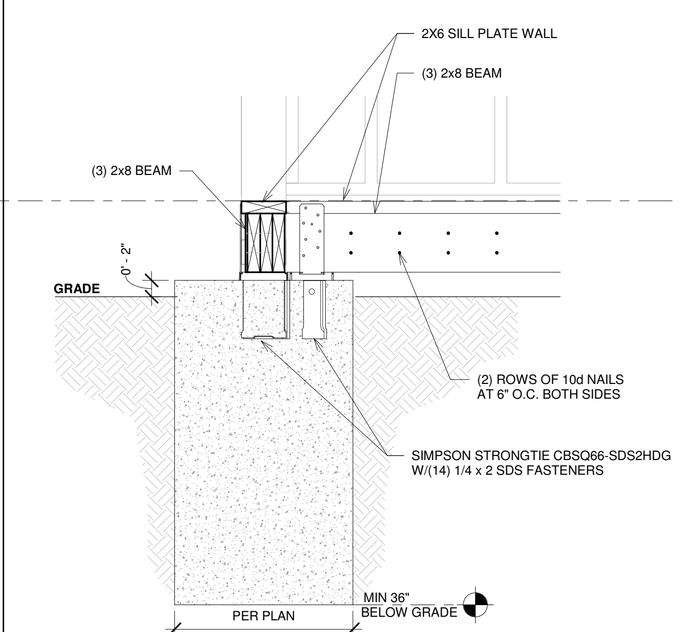
5 CORNER CARPORT PIER SCALE: 1" = 1'-0"
