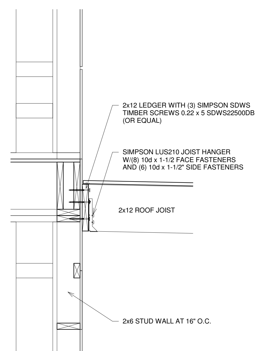
4 BALCONY FLOOR JOISTS SCALE: 1" = 1'-0"
