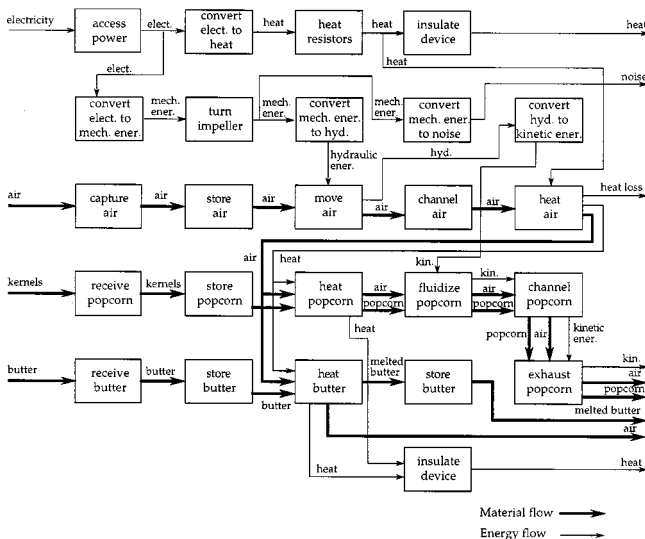
Fig. 6 Functional model of the hot air popcorn popper generated without a structured vocabulary (FM A)
