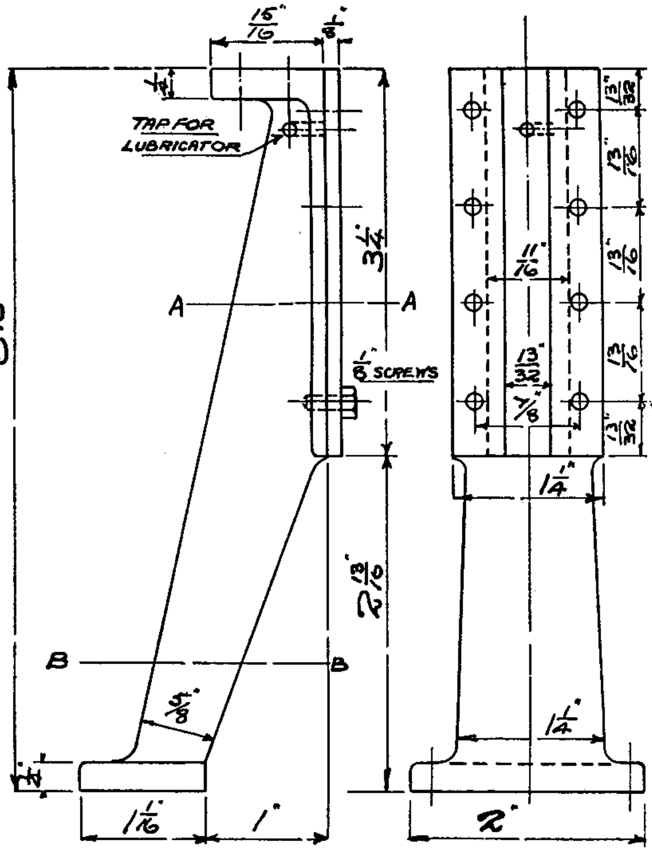
BACK COLUMNS. 2 OFF. CAST IRON. MILD STEEL GUIDE PLATES.
