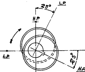
LAP 1/16 LEAD 1/64 THROW 3/16
