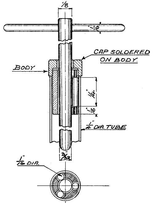
Three Roller Type Tube Expander
