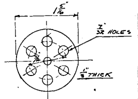
VALVE SEAT.
