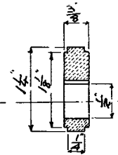
ECCENTRIC SHEAVES, 2 OFF, MILD STEEL.
