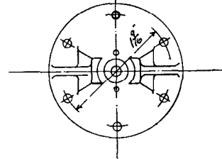
PUMP COVER
