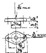
GLAND.
