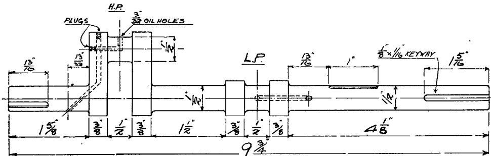
CRANK SHAFT 1 OFF, MILD STEEL
