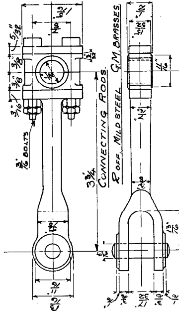
SOME DETAILS OF COMPONENTS OF MODEL COMPOUND CONDENSING STEAM ENGINE.
