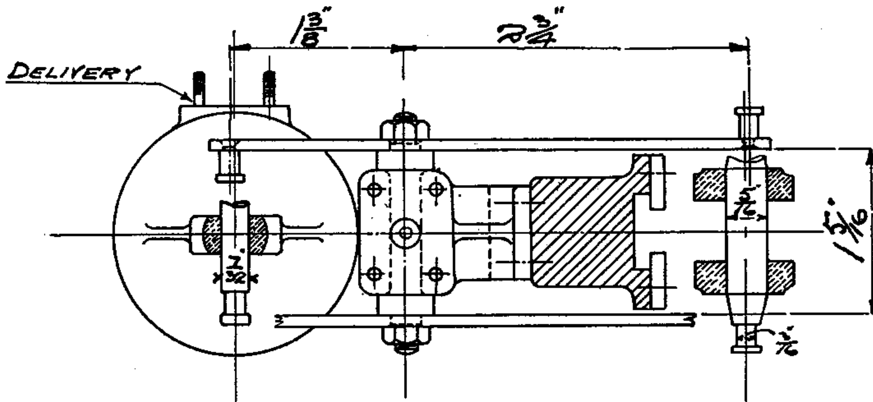
ARRANGEMENT OF PUMP LEVERS
