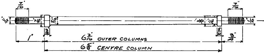
FRONT COLUMNS, 3 OFF, MILD STEEL
