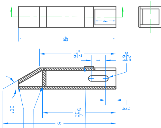
Cross-over Tube (2 x 2 x 0.188 wall)
